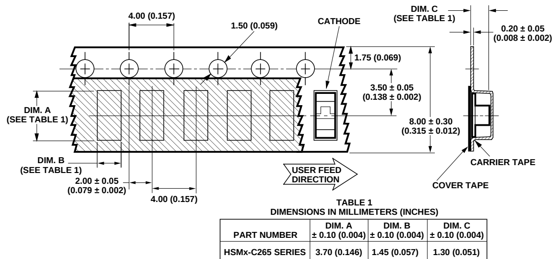
Figure 16. Tape dimensions.
