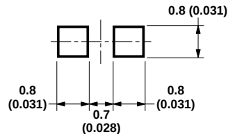
Figure 12. Recommended soldering pattern for HSMx-C190, HSMx-C191 and HSMx-C197.
