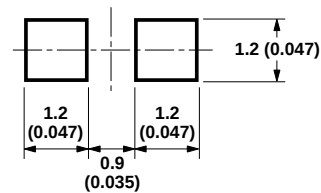
Figure 11. Recommended soldering pattern for HSMx-C170 and HSMx-C177.
