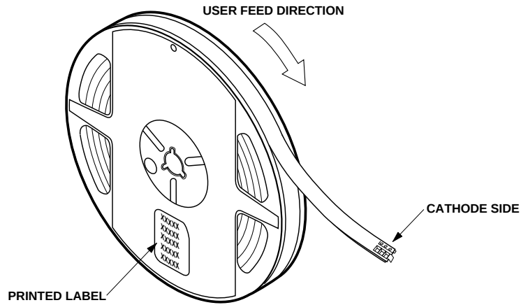
Figure 14. Reeling orientation.
